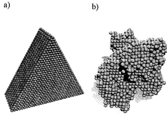
FIGURE 8 (a) Rough shell triangular model of BSA with dimensions of 80 \times 80 \times 80 \times 30 Å; (b) Rough shell model derived from the atomic-level structure of HSA (PDB file 1bm0; Sugio et al., 1999)
