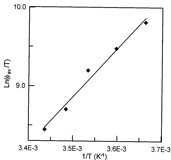
FIGURE 6 Plot of \ln(\phi_{\text{av}}/T) versus 1/T (Eq. 11 in the text) for the erythrosin-BSA complex in glycerol/buffer ( 10^{-6} M, 92% w/w).
