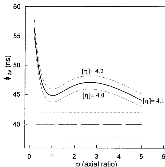
FIGURE 7 The expected average correlation time \phi_{av} (1 cP, 20^\circ\text{C} ) of ellipsoidal models of BSA as a function of the axial ratio p (oblate p < 1 and prolate p > 1 ). The values of \phi_{av} were computed from Eq. 12, keeping constant the protein intrinsic viscosity [\eta] = 4.1 \pm 0.1 \text{ cm}^3 \text{ g}^{-1} , as described in the text. The rotational correlation time expected for the elongated model ( p = 3.5 ) of Fig. 1 a is \sim 46 \text{ ns} , which differs significantly from the experimental value ( 40 \pm 2 \text{ ns} ), indicated here by the horizontal lines.
