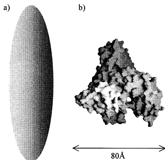
FIGURE 1 (a) The elongated ellipsoid ( 140 \times 40 Å) used frequently to model the conformation in solution of human and bovine serum albumin; (b) An image of HSA at the same scale, adapted from the Brookhaven Protein Data Bank x-ray coordinates file 1bm0 (Sugio et al., 1999).
